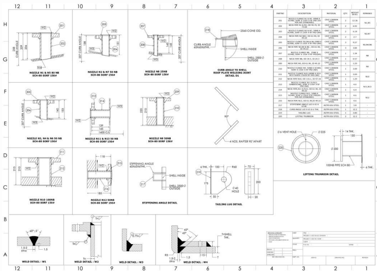
Pressure Vessel Drawings
